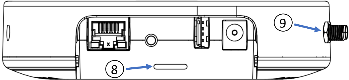
Figure 3 – Cascade-500-W/X Gateway – Back View
